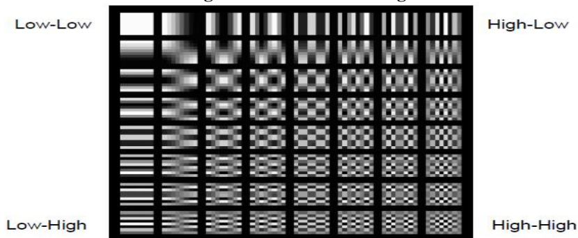
Figure 4: DCT Coefficients
