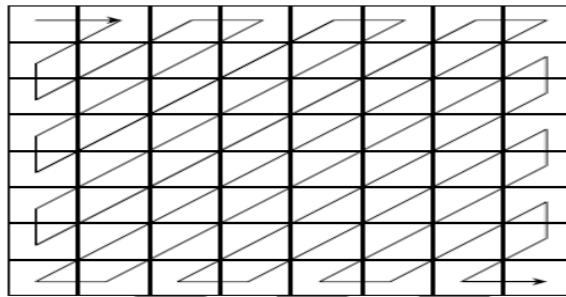
Figure 2: zigzag ordering of DCT coefficients
